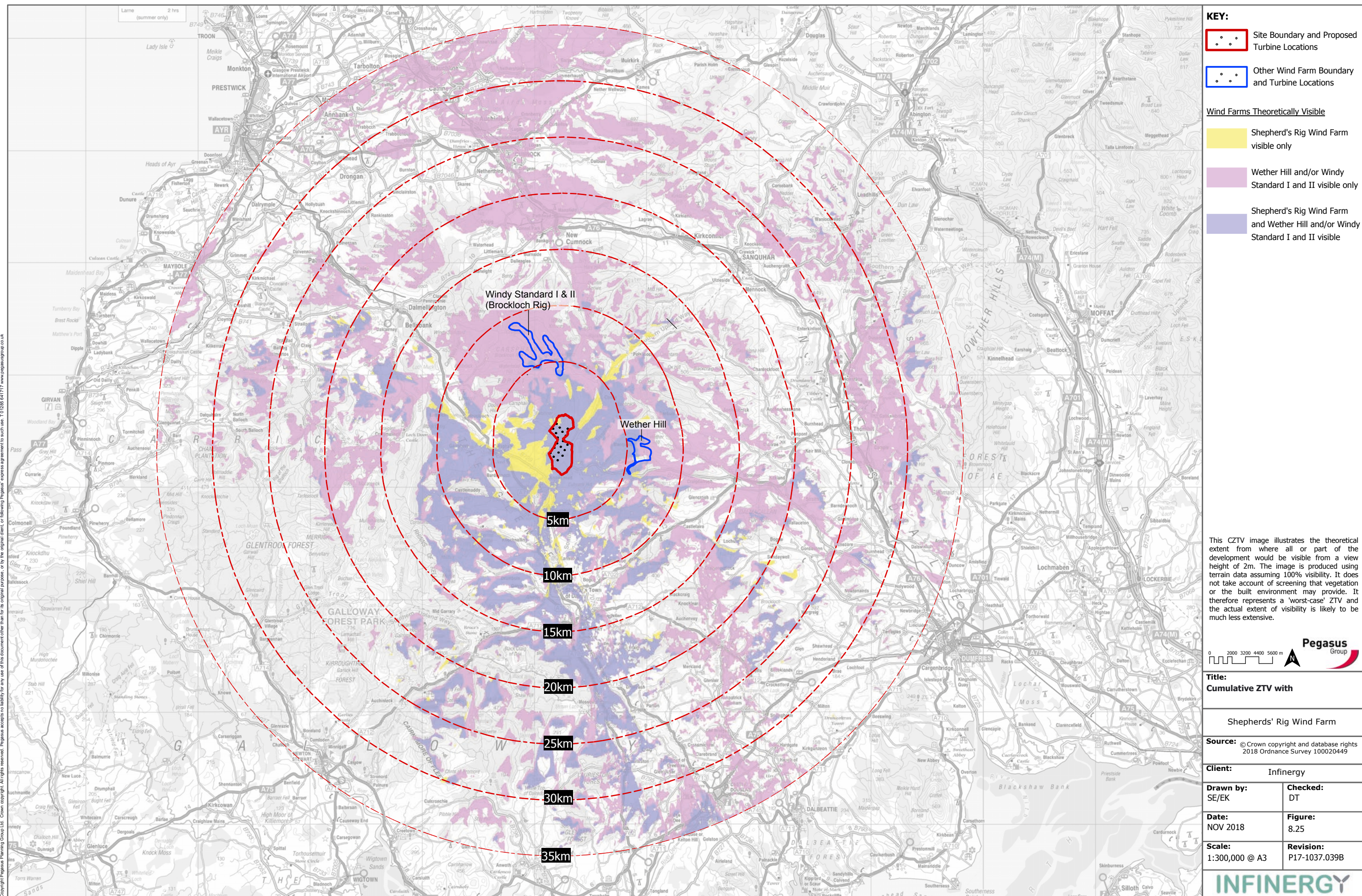
Figure 8.25: Cumulative ZTV with Wether Hill and Windy Standard I and II
